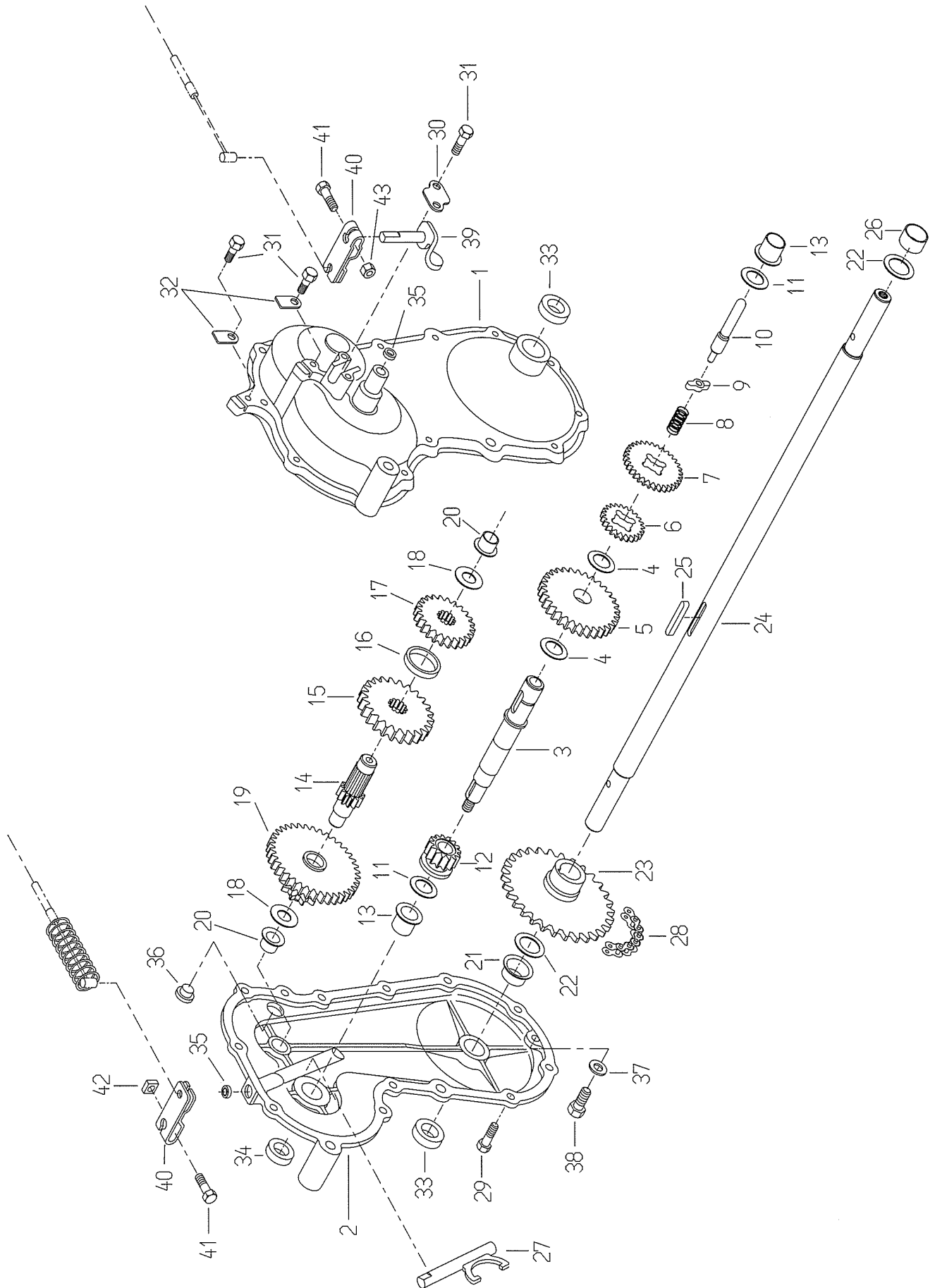
Fig. 2 TRANSMISSION
