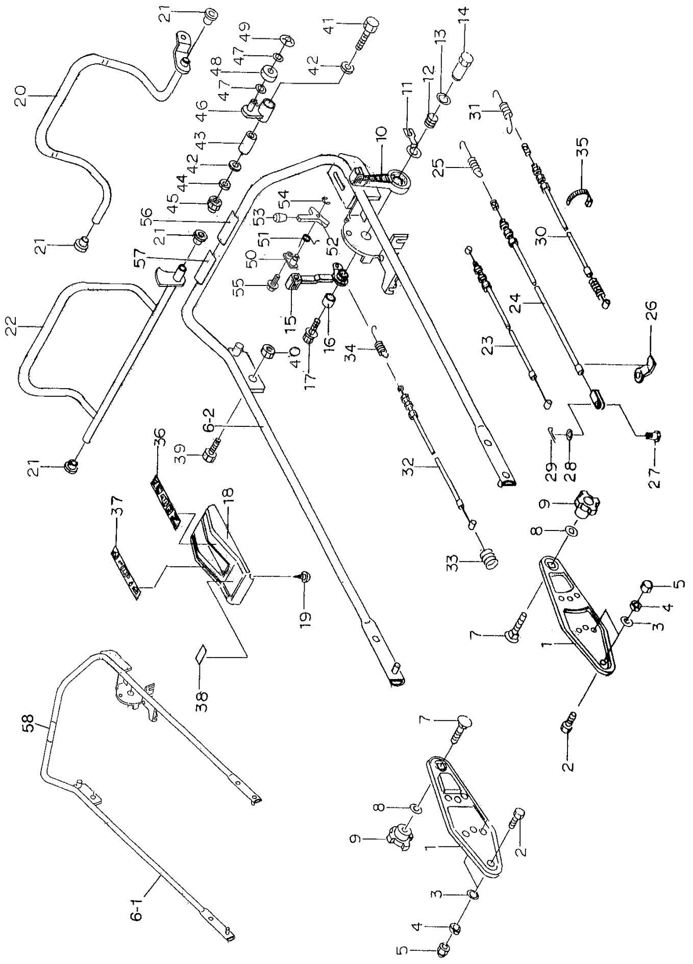
Fig 5 Handle
